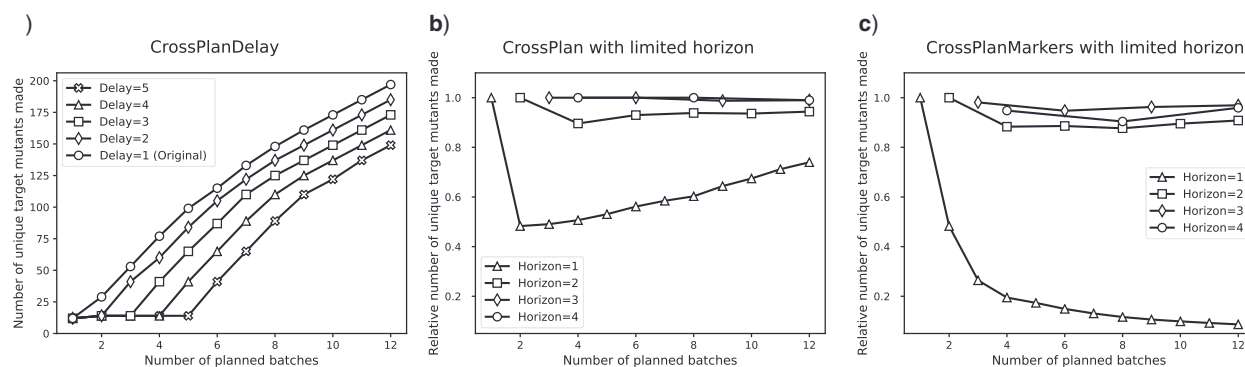
Fig. 5. Variation with k of (a) number of mutants planned by CrossPlanDelay, (b) the ratio of the number of target mutants planned by the limited horizon strategy and the number planned by CrossPlan and (c) the ratio of the number of target mutants planned by the CrossPlanMarkers with the limited horizon strategy and the number planned by CrossPlan
